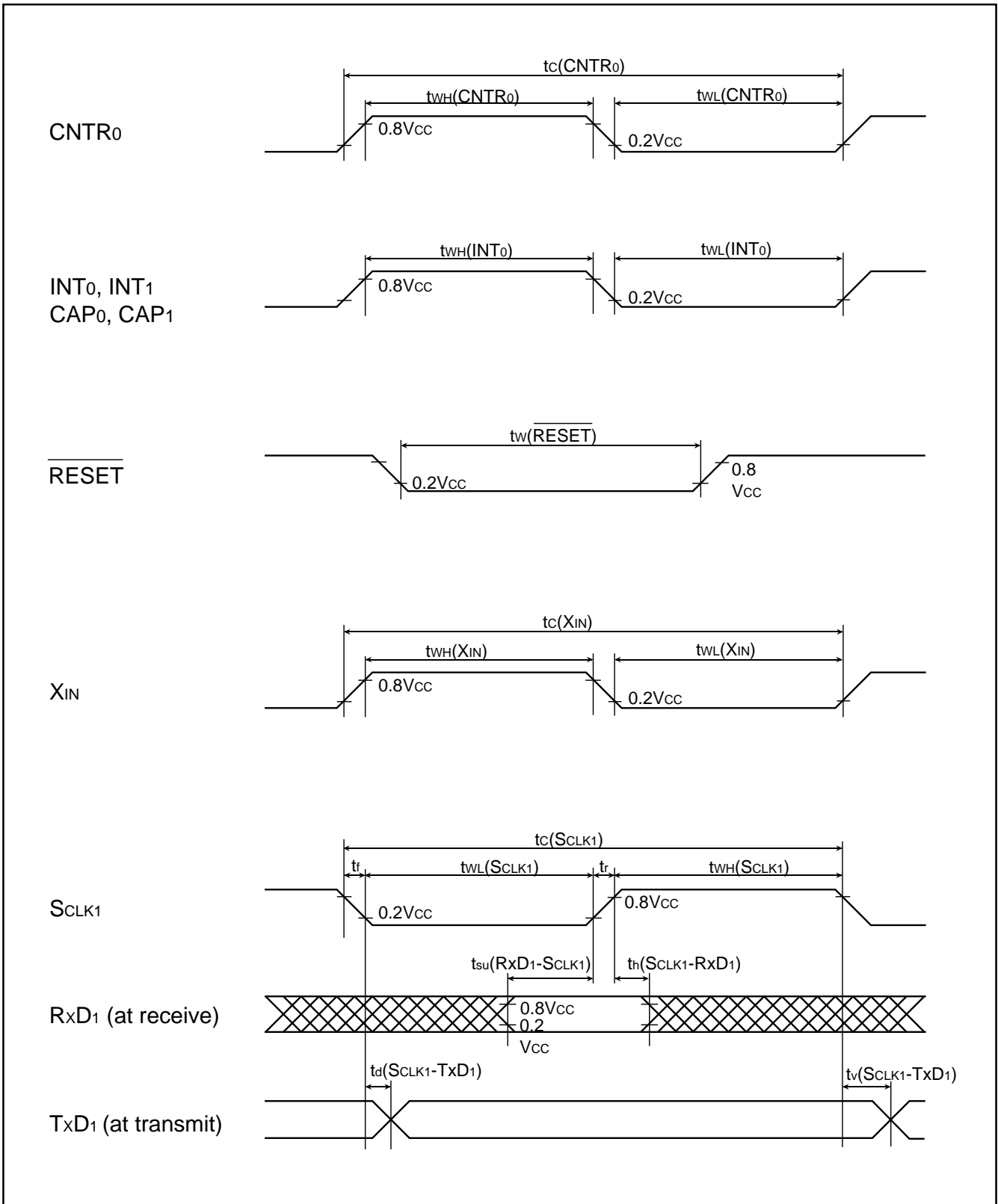
Fig. 95 Timing chart
