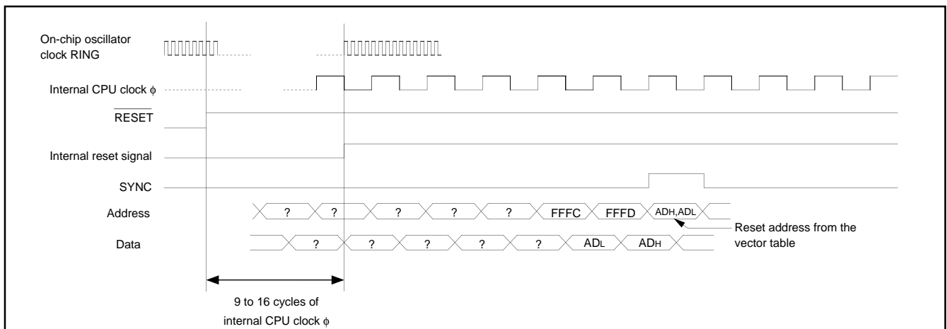
Fig. 69 Timing diagram at reset
